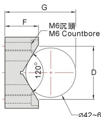
V型鉗口(A型B型用) V-Clamp(for MKS-A & B)
